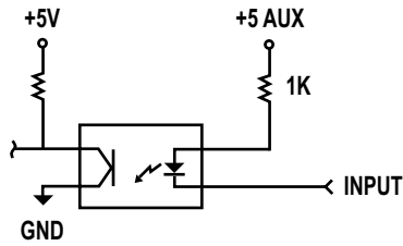
Figure 1 - Logic Input Circuit (Enable, DTS)
